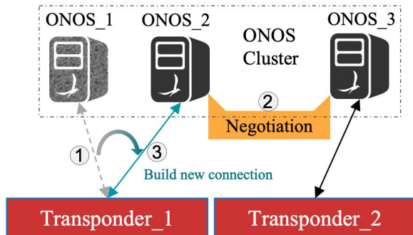
Fig. 3 Mastership movement in ONOS cluster.
