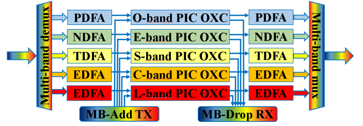
Fig. 2. Possible architecture for a MB ROADM.
