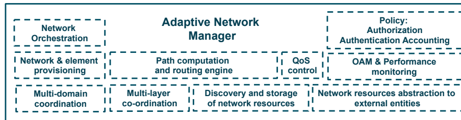
Figure 3: ANM functional building blocks
